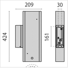
000442 Wall bracket 45
