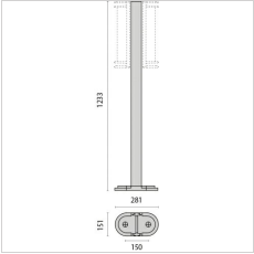
000454 Post 45 H1200
